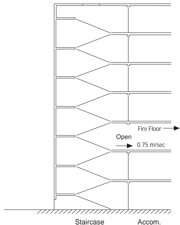
Fig 5 - Velocity Criterion
